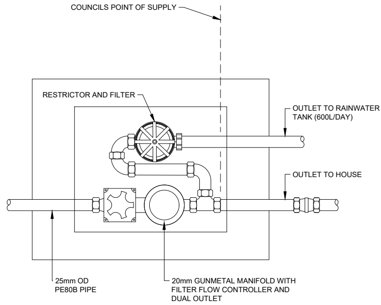
MANIFOLD - PLAN VIEW
