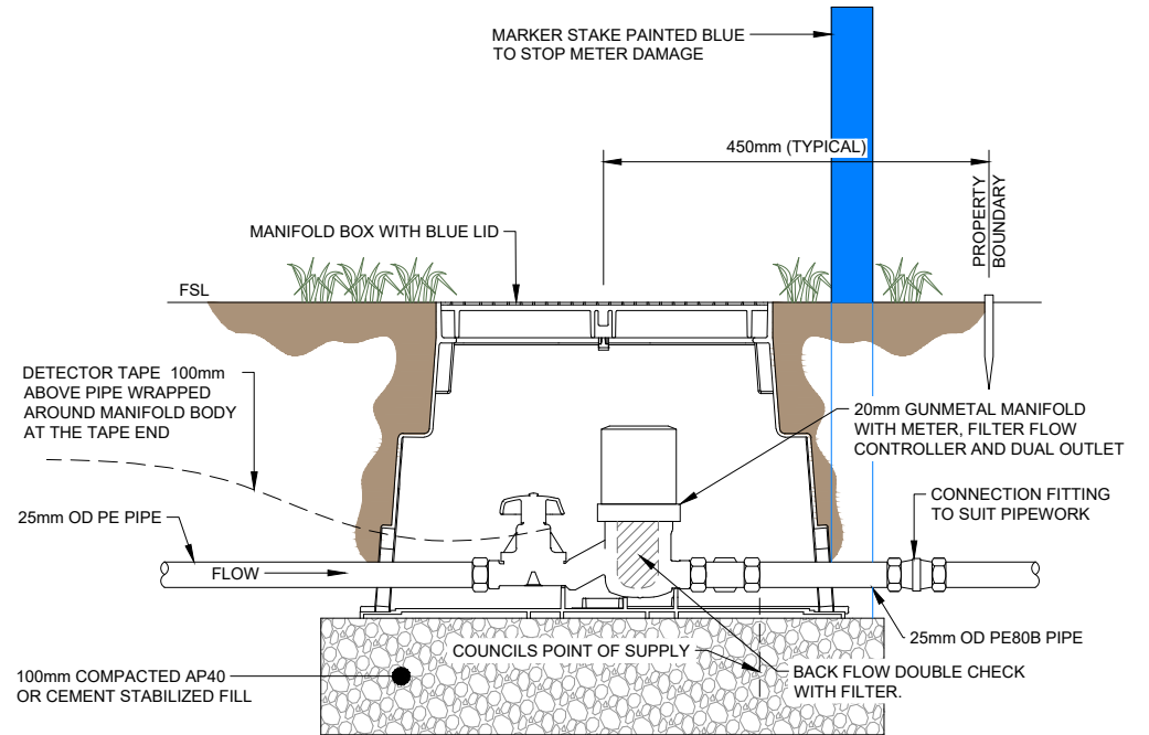
MANIFOLD - ELEVATION
