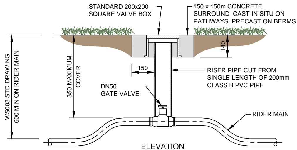
GATE VALVE
