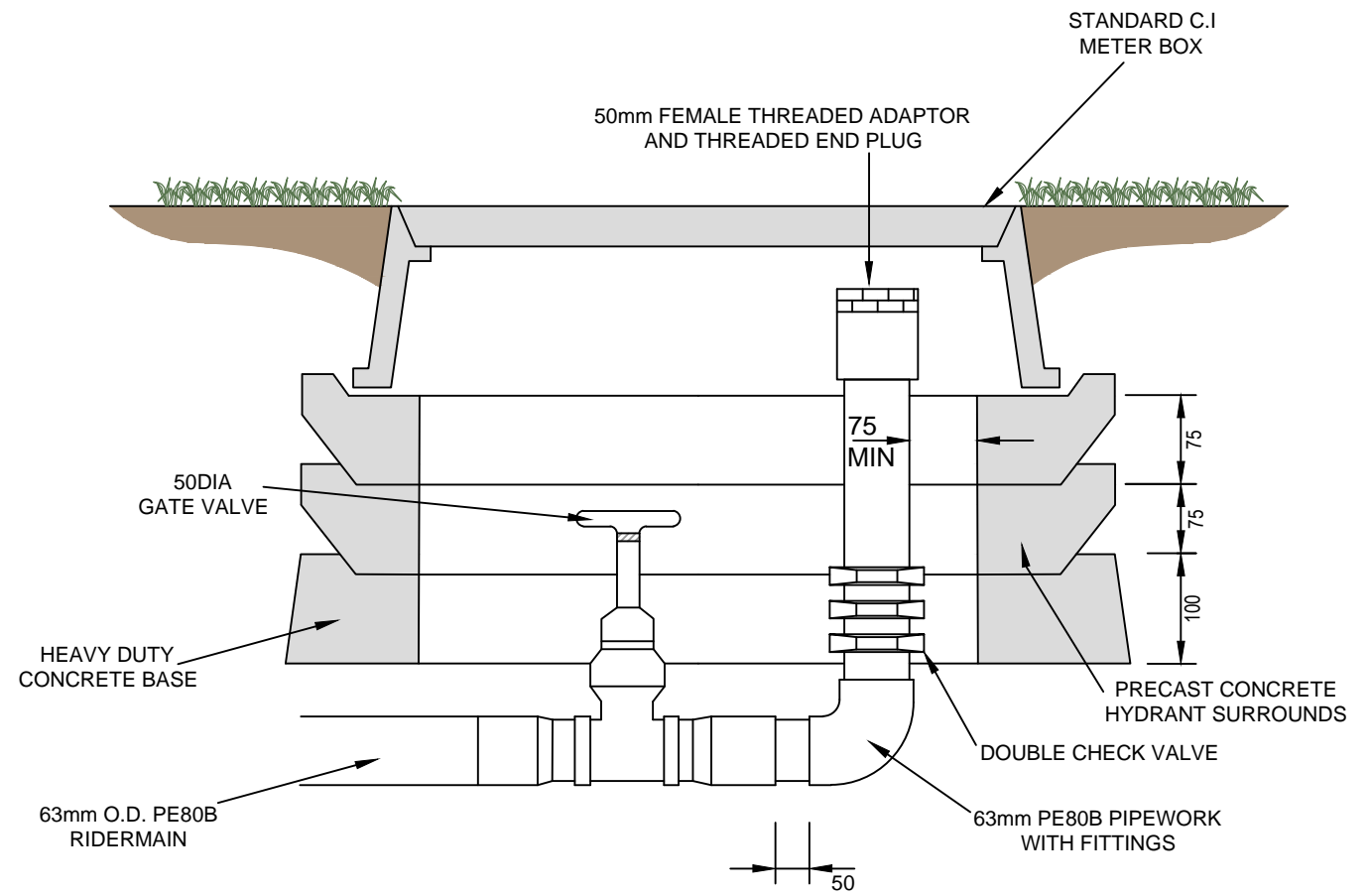
FLUSHOUT AT END OF RIDERMAIN
