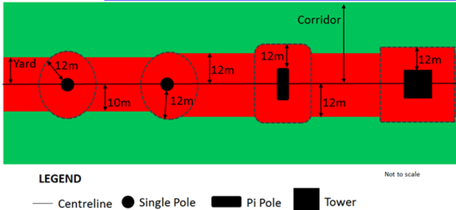
Diagram 1: National Grid Corridor and National Grid Yard
