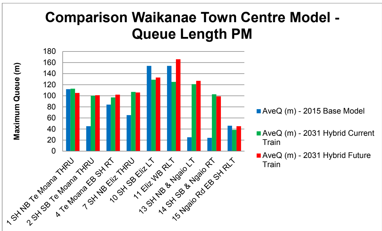
Figure 5.3.7 – Queue Length Comparison Graph – 2031 PM Peak (Current vs Future Train Timetable)
