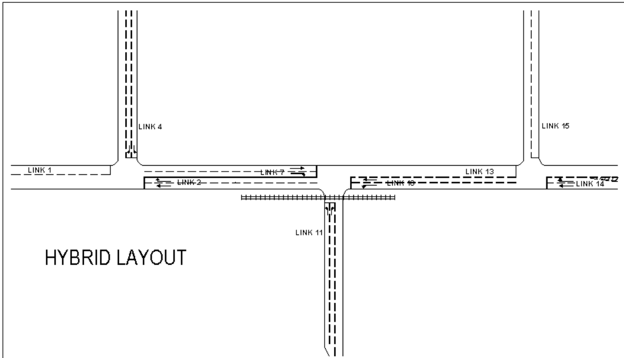
Figure 5.2.3 – Hybrid Lane Arrangement
