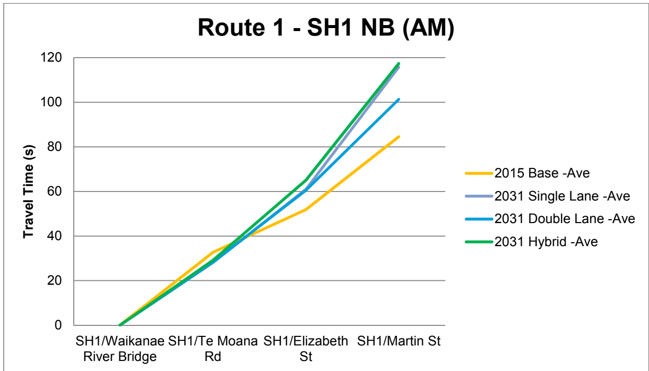
Figure 5.2.8 - Route 1 SH1 Northbound AM Peak Journey Time Graph
