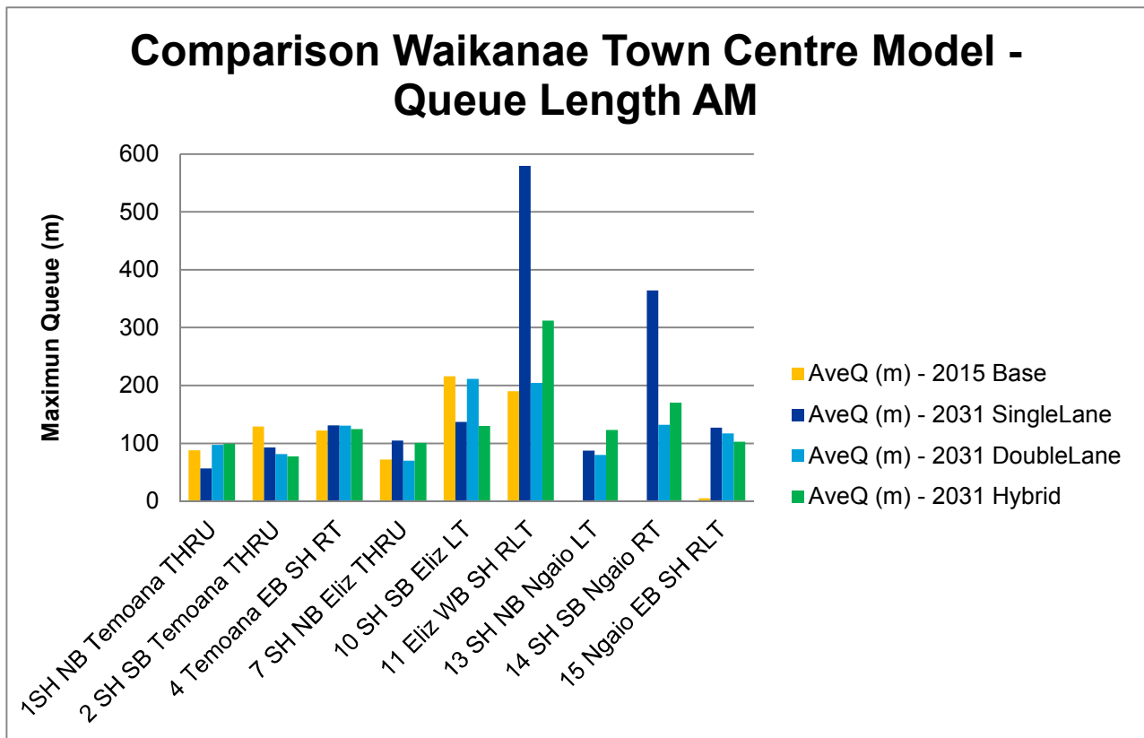
Figure 5.2.4 & 5 - Queue Lengths in AM Peak
