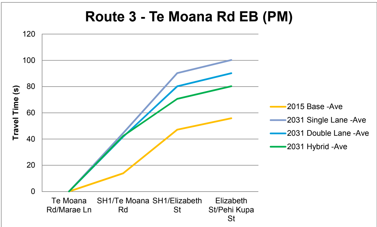
Figure 5.2.14 - Route 3 Te Moana Road to Elizabeth Street PM Peak Journey Time Graph
