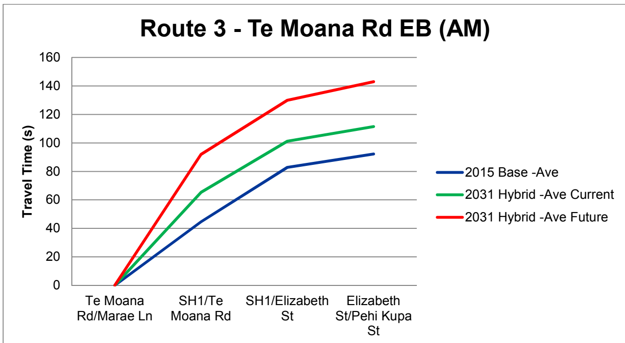
5.3.1 – Route 3 Te Moana Road to Elizabeth Street AM Peak Journey Time Graph (Current vs Future Train Timetable)
