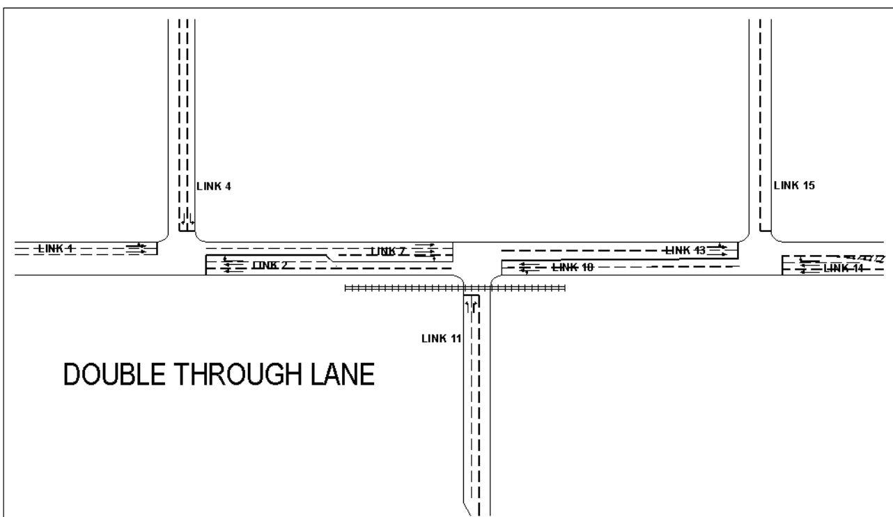
Figure 5.2.2 – Two Lane Arrangement
