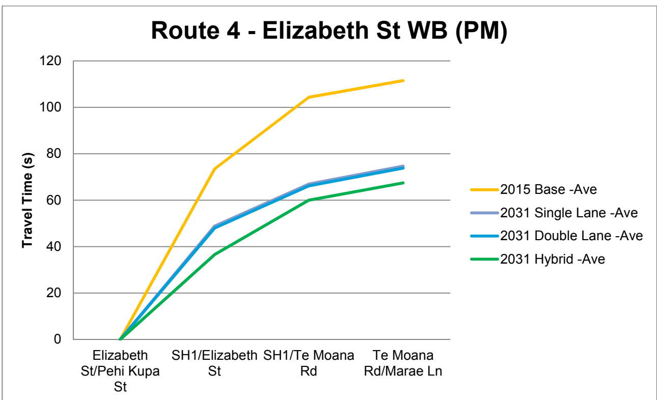
Figure 5.2.15 - Route 4 Elizabeth Street to Te Moana Road PM Peak Journey Time Graph
