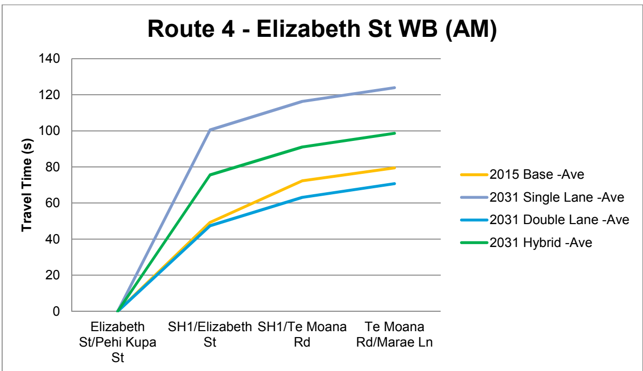
Figure 5.2.11 - Route 4 Elizabeth Street to Te Moana Road AM Peak Journey Time Graph
