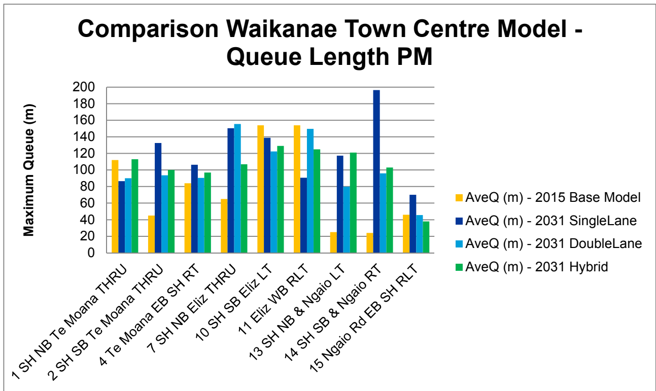
Figure 5.2.6 & 7 - Queue Lengths in PM Peak
