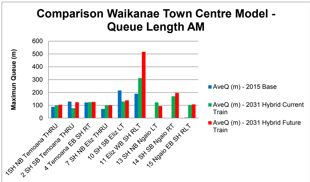
Figure 5.3.6 – Queue Length Comparison Graph – 2031 AM Peak (Current vs Future Train Timetable)
