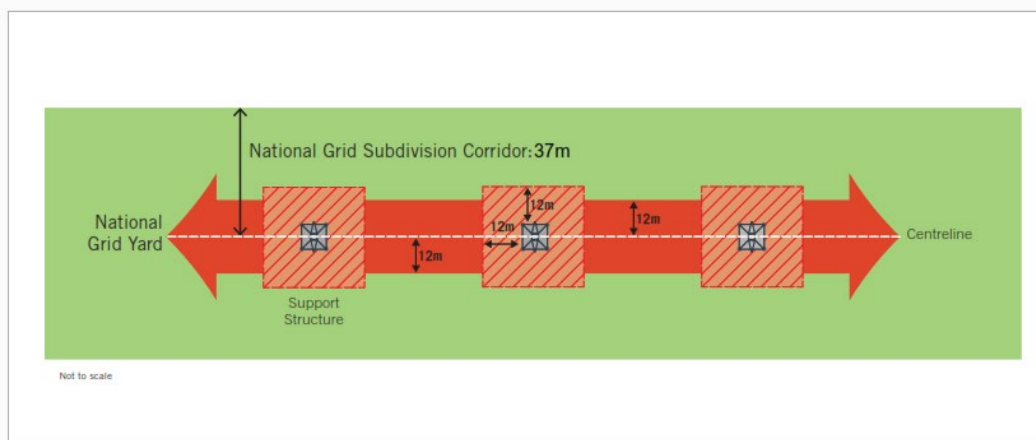
Diagram 1: National Grid Subdivision Corridor and National Grid Yard
