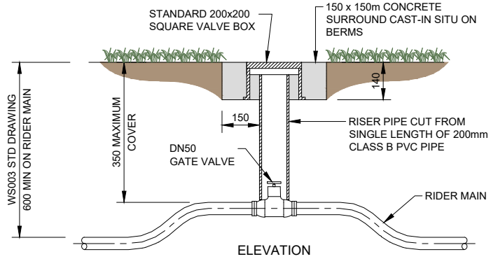
GATE VALVE
