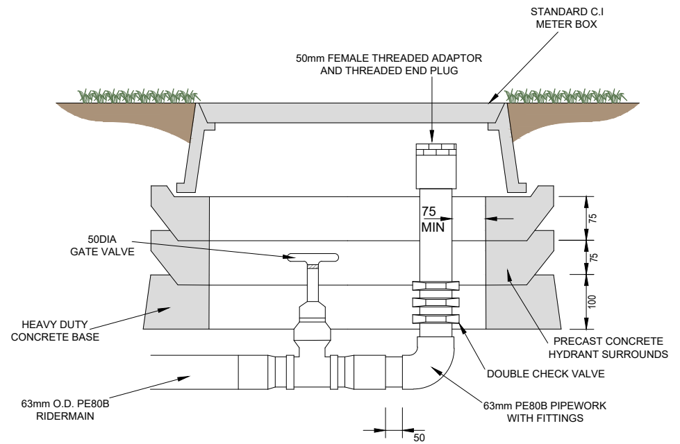
FLUSHOUT AT END OF RIDER MAIN
