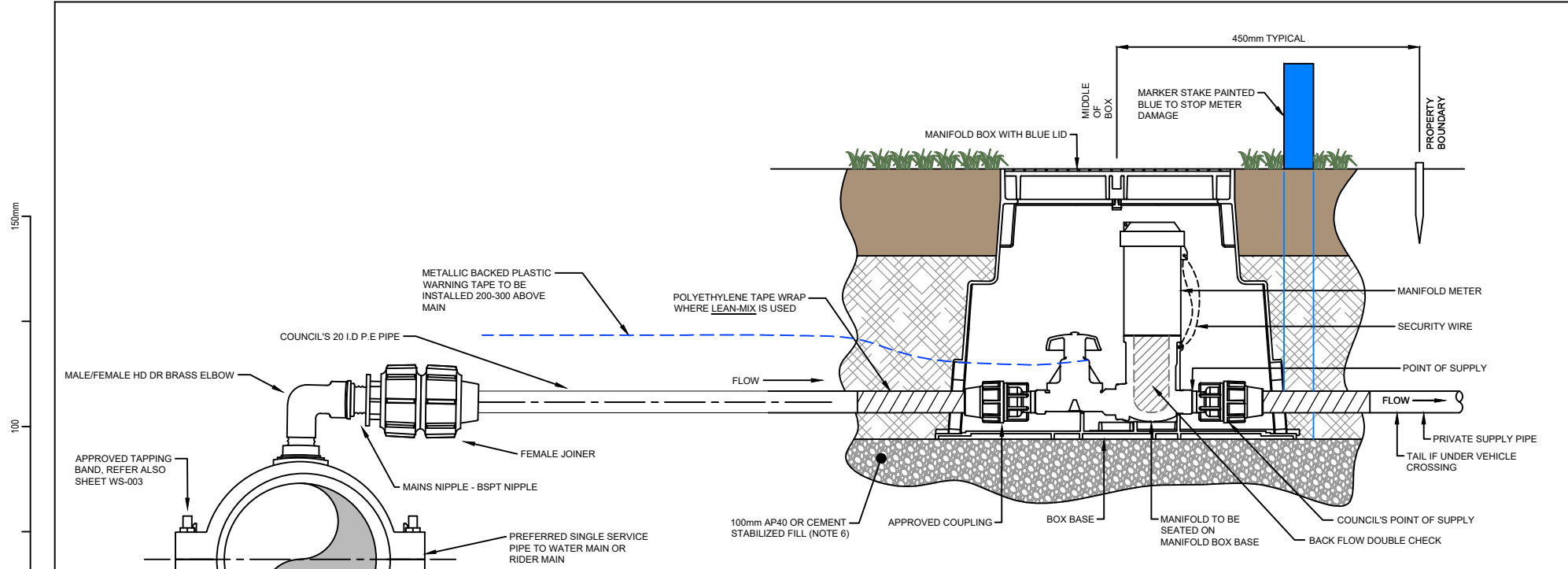
STANDARD MANIFOLD INSTALLATION
