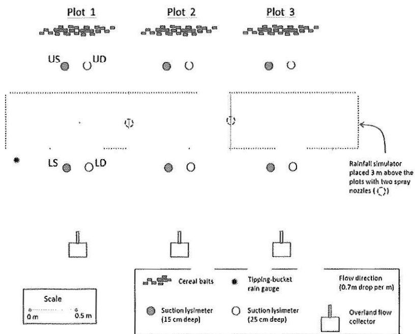
Figure 4-2: Schematic of plot and instrumentation arrangement - plot-scale study.
