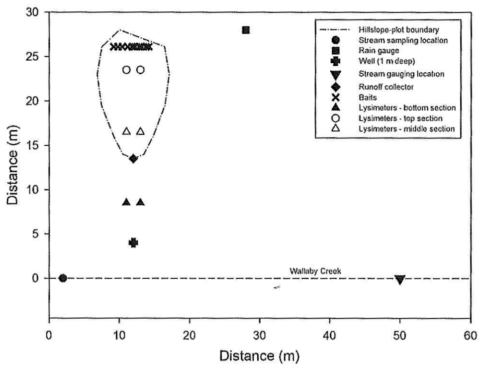
Figure 5-1: Schematic of hillslope-scale study site.
