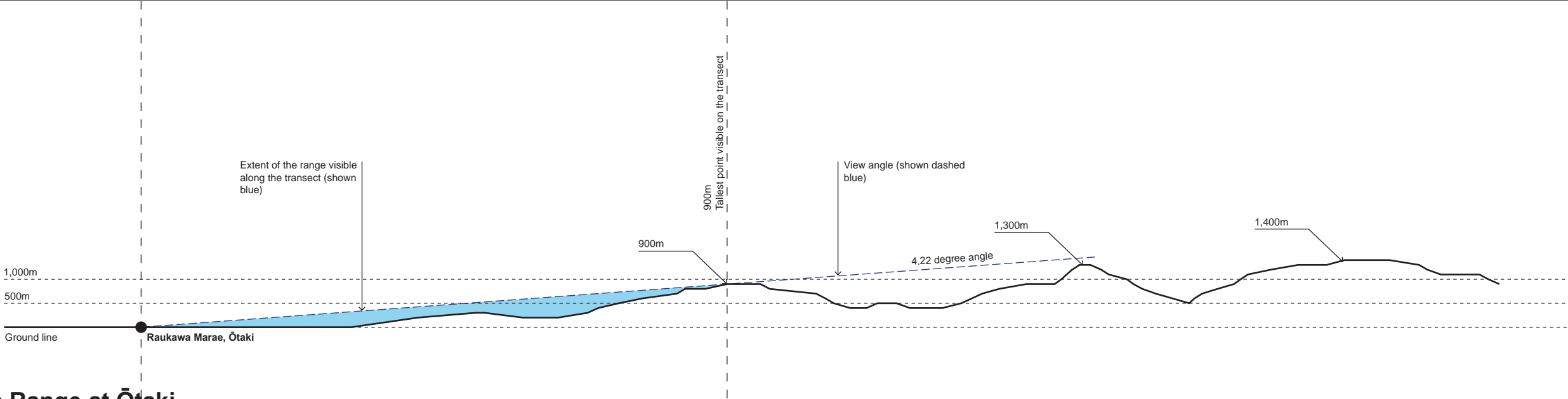
Transect through the Tararua Range at Ōtaki
