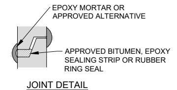
DETAILS OF STEPPED IRONS NOTE: STEPPED IRONS SHALL BE 20 Ø GRADE 316 STAINLESS STEEL OR APPROVED ALTERNATIVE
