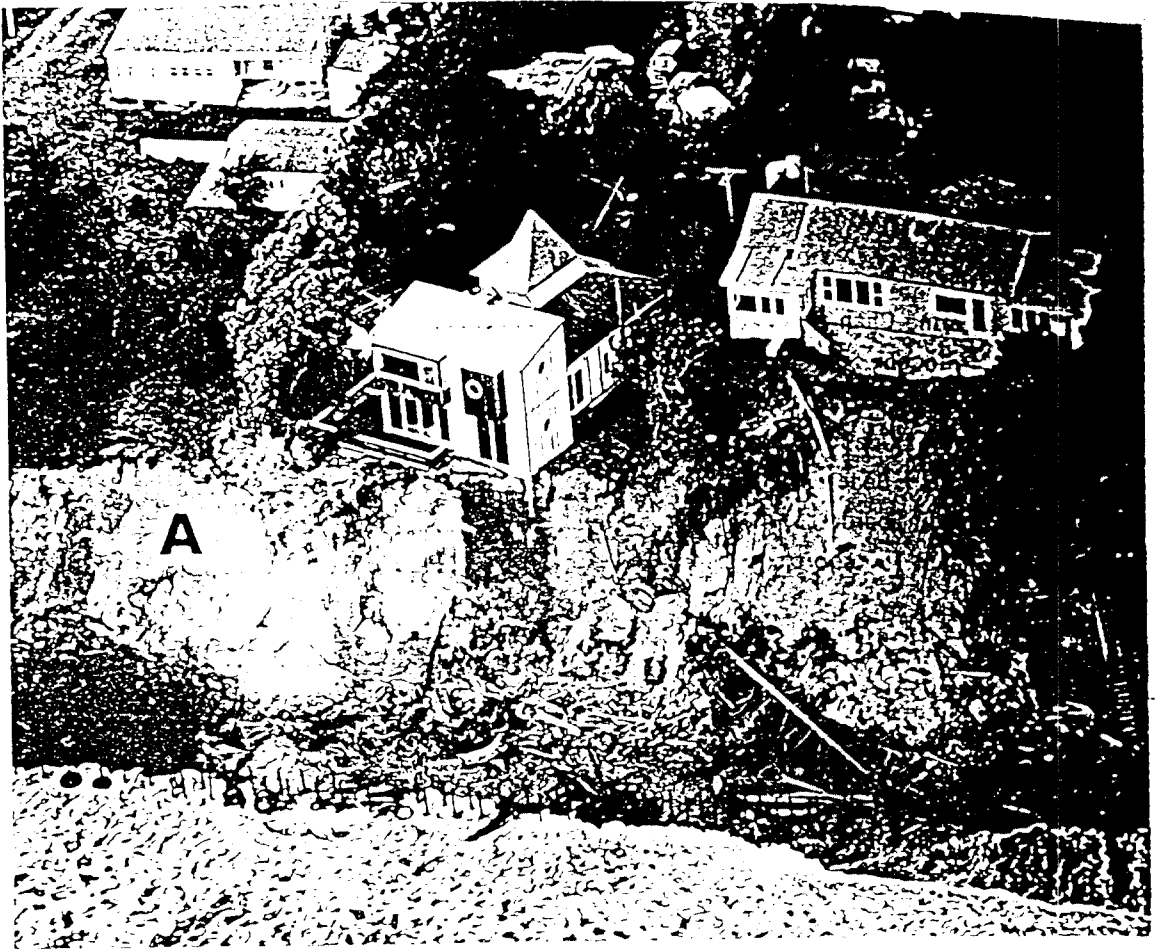
FIG. 1 Coastal erosion and protection at Ramati Beach, "Golden Coast".
