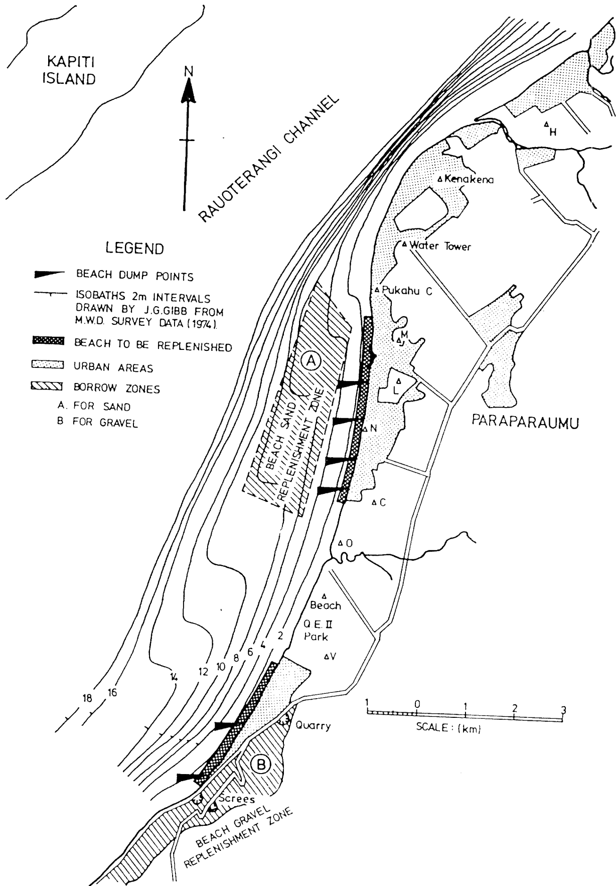
FIG. 11 Sources of sand and gravel for artificial beach replenishment at Paekakariki and Raumati. Possible dumping points are indicated so that quantities placed on the beach can be distributed alongshore by longshore currents.
