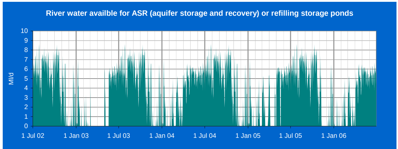
Figure 9-3: River Water Available for Recharging the Aquifer for ASR
