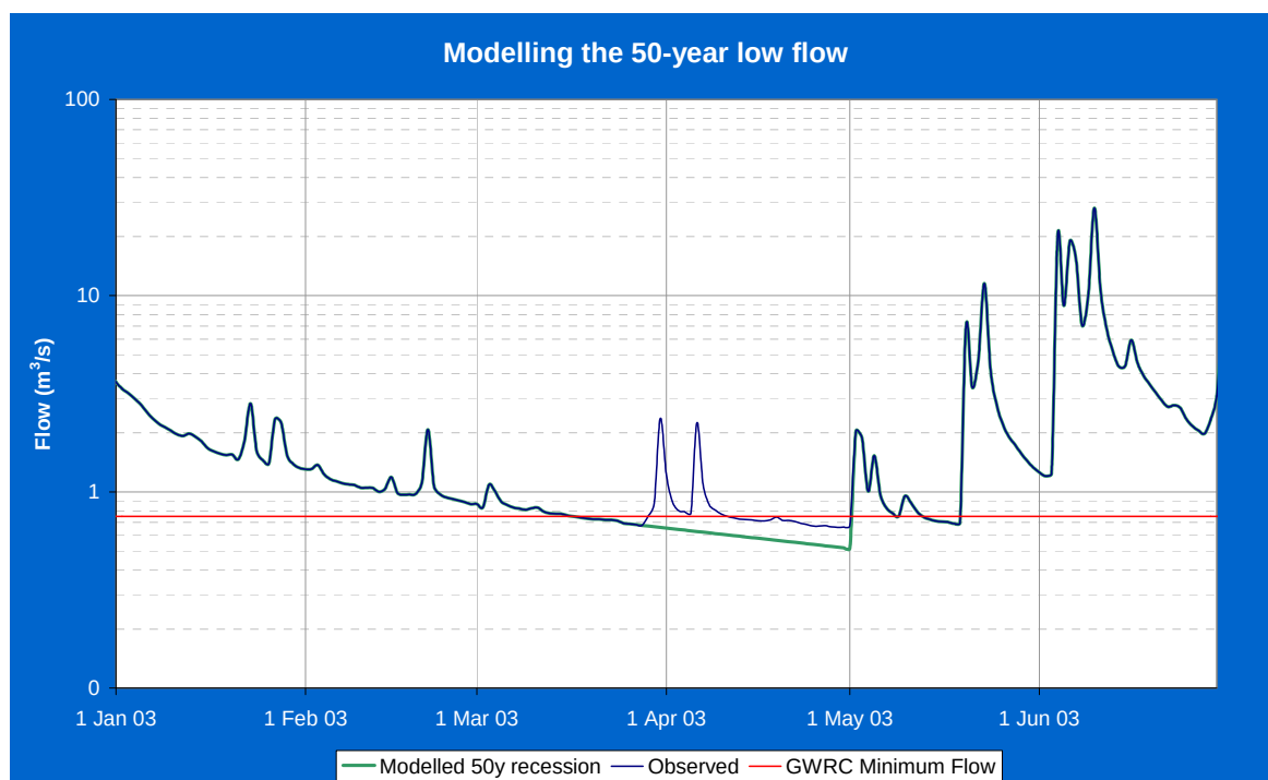
Figure 3-2: Modelled 50 Year Low Flow
