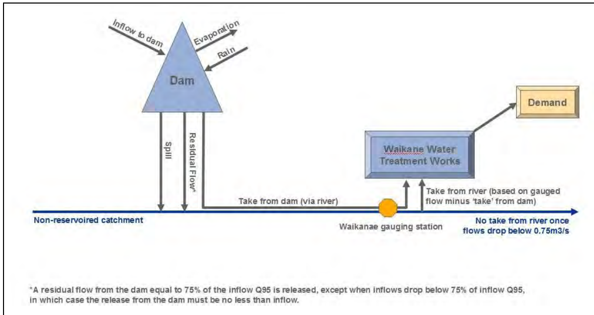
Figure 3-4: Dam Options Modelling Schematic
