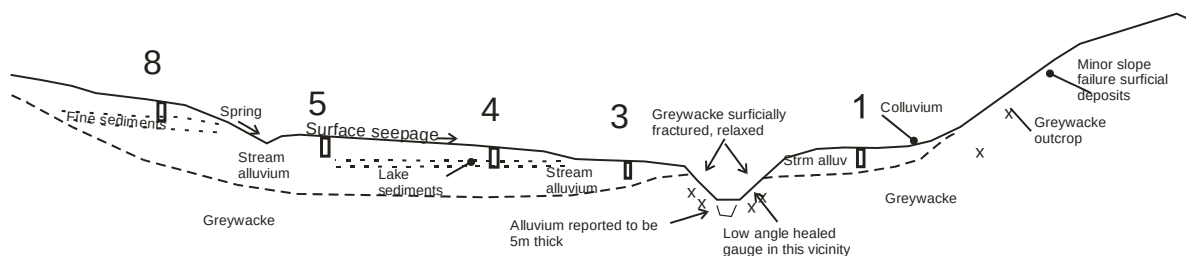
Figure 4-5: Geologic Profile Along the Upper Dam Site Axis Looking Downstream
