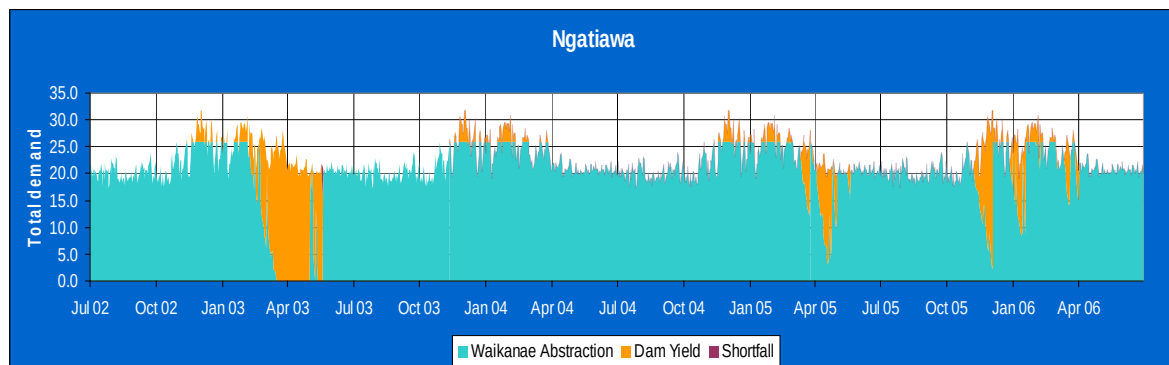
Figure 6-4: Yield to meet demand with Ngātiawa Dam (1.5M m 3 )
