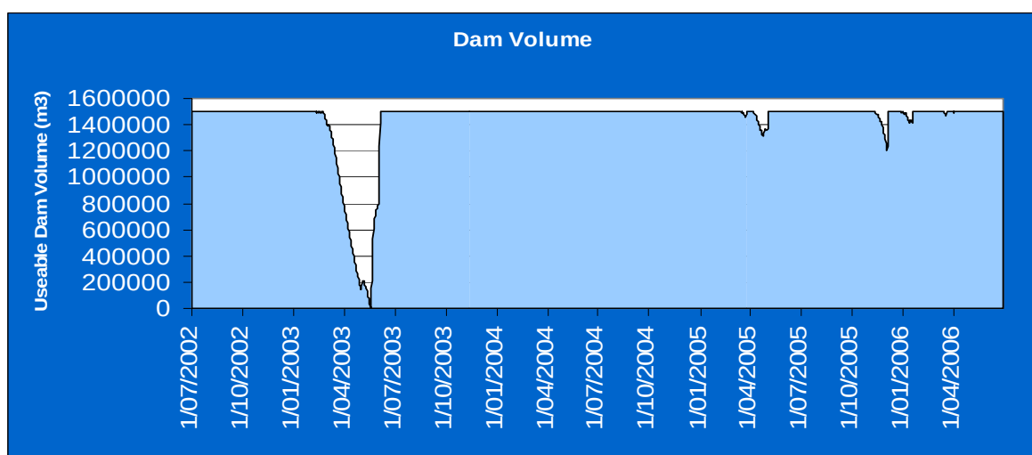
Figure 6-5: Ngātiawa Dam (1.5M m 3 ) Volume Profile for 50-year Drought
