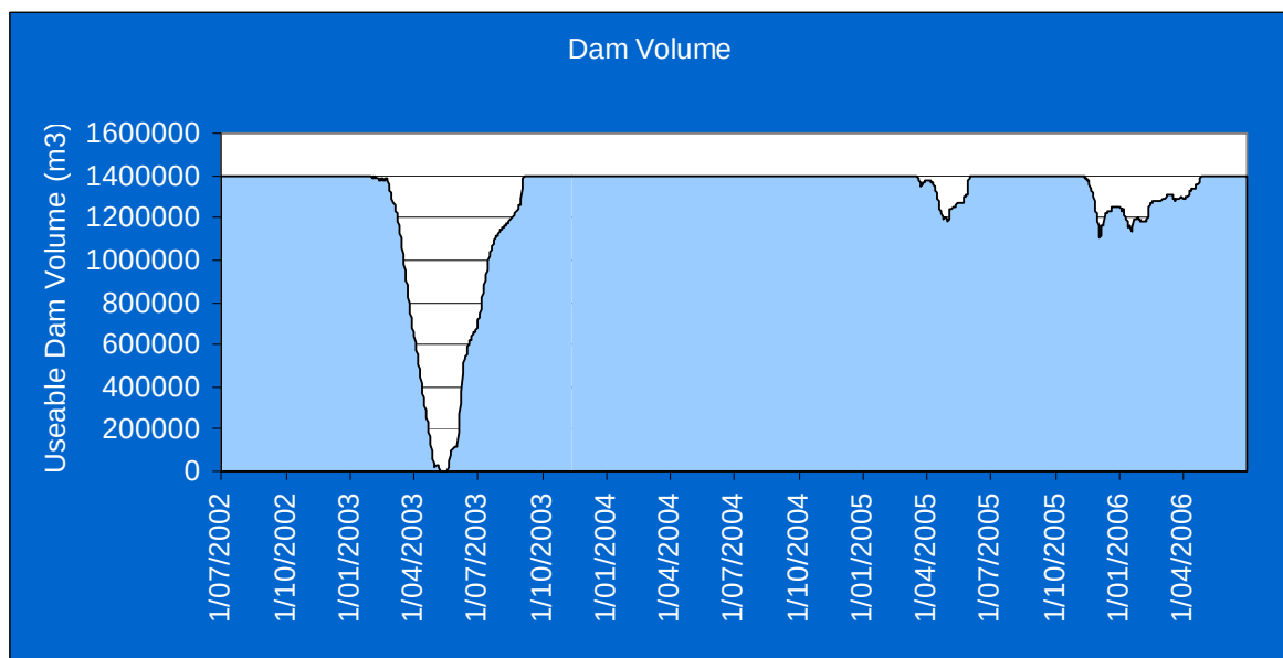
Figure 4-9: Kapakapanui Dam (1.4M m 3 ) Volume Profile for 50-year Drought
