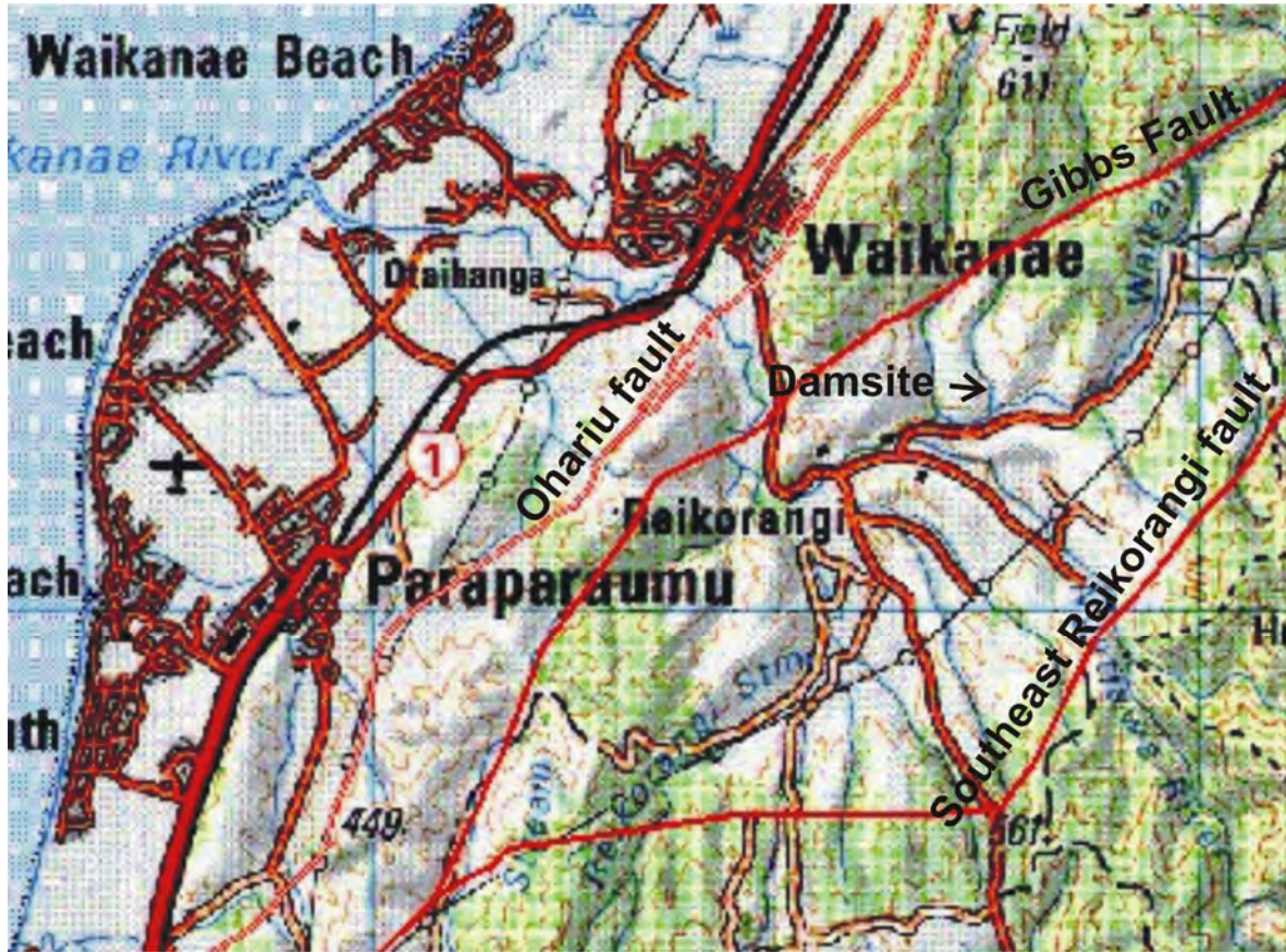
Figure 4-6: Active Faults in the Vicinity of Kapakapanui Dam
