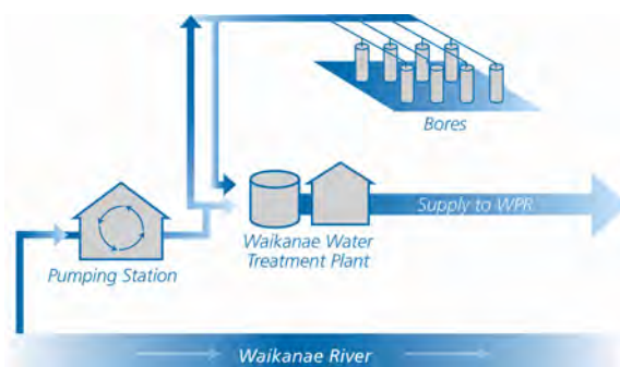
Figure 8-1: Waikanae Borefield and Treatment Option Schematic
