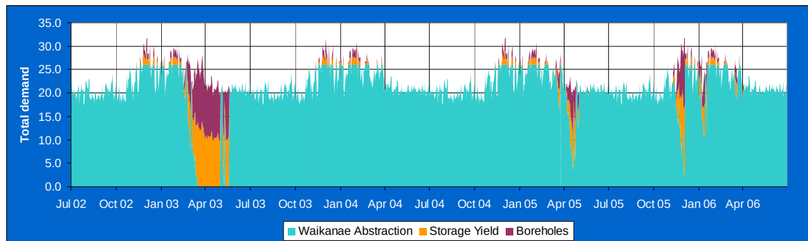
Figure 7-5: Yield to meet demand with Borefield and Storage Ponds Scenario 1
