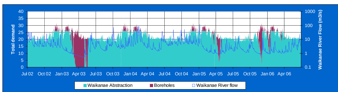
Figure 8-3: Yield to meet demand with Extended Borefield
