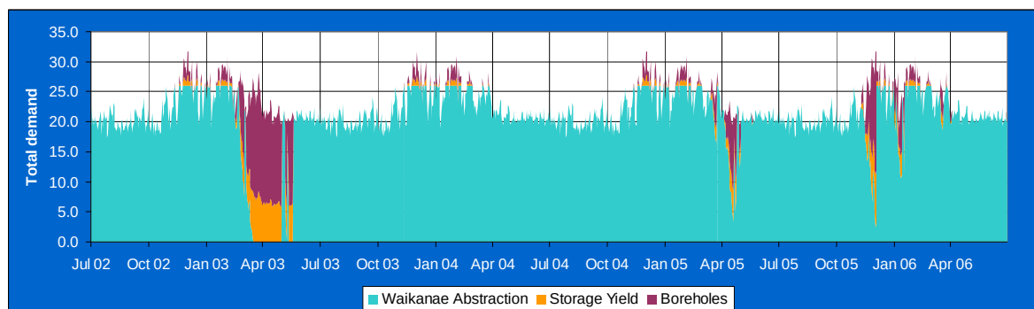
Figure 7-6: Yield to meet demand with Borefield and Storage Ponds Scenario 2
