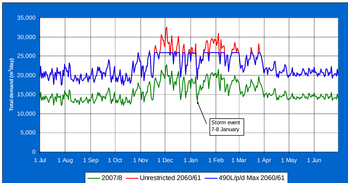
Figure 3-3: Annual Demand Profiles used in Yield Modelling
