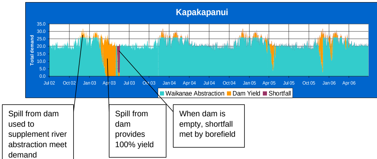
Figure 4-8: Yield to Meet Demand with Kapakapanui Dam (1.4M m 3 )
