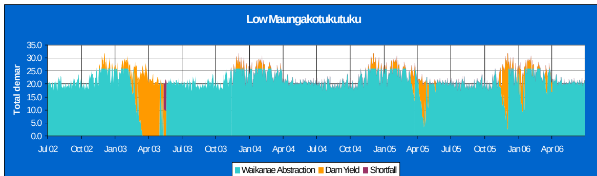
Figure 5-5: Yield to meet demand with Lower Maungakotukutuku Dam (1.4M m 3 )
