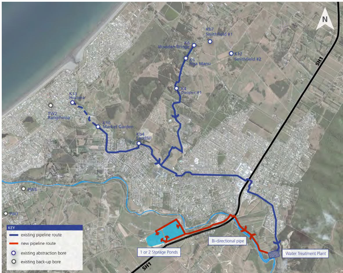
Figure 7-2: Storage Pond Site Location
