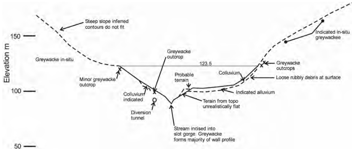
Figure 5-3: Geologic Profile Along Dam Axis Looking Downstream
