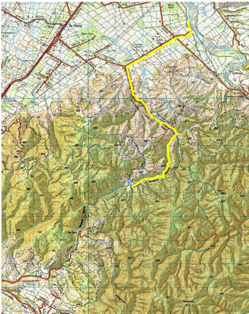
Figure 14-3: Ōtaki River Transfer – Pipeline Route
