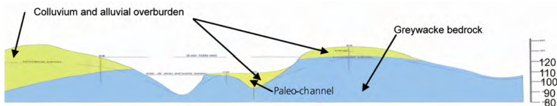
Figure 4-2: Geologic Profile Along the Lower Dam Site Axis Looking Downstream
