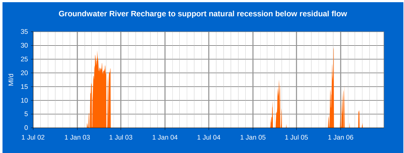
Figure 10-4: Discharge to River for River Recharge with Groundwater Scheme
