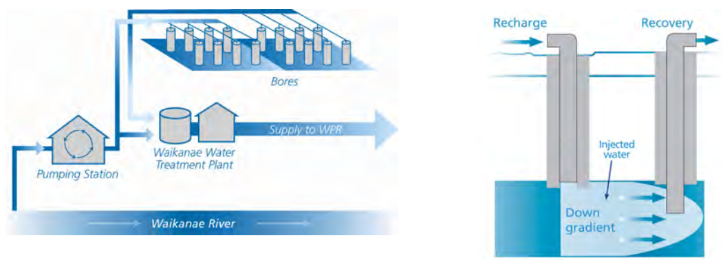
Figure 9-1: Aquifer Storage and Recovery Schematics
