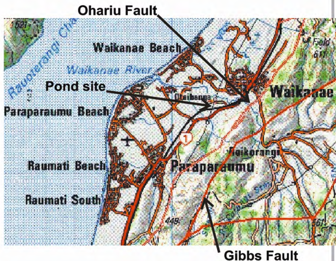
Figure 7-4: Active Faults in the Vicinity of Storage Pond Site 24
