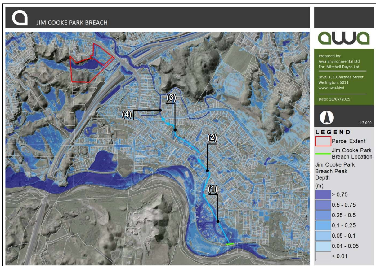
Figure 6 Jim Cooke Park Stop-Bank Breach Scenario Peak Depths
