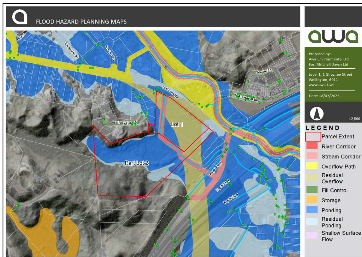
Figure 3 Flood Hazard Planning Maps Overlain Lots
