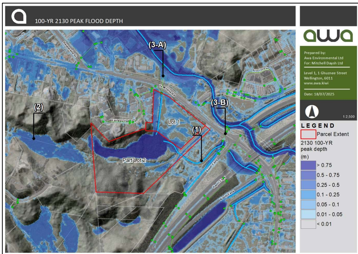
Figure 4 100-YR 2130 Existing Peak Inundation
