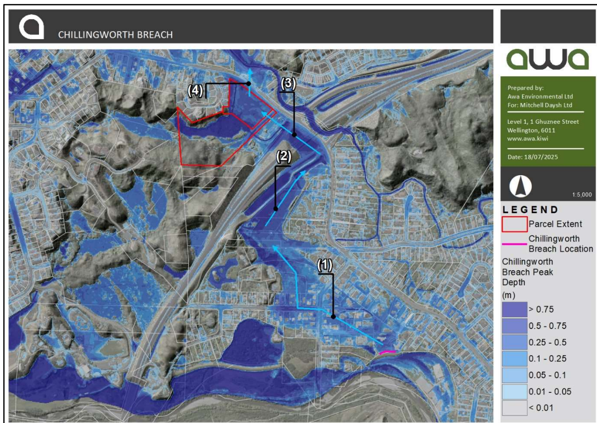
Figure 7 Chillingworth Stop-Bank Breach Scenario Peak Depths
